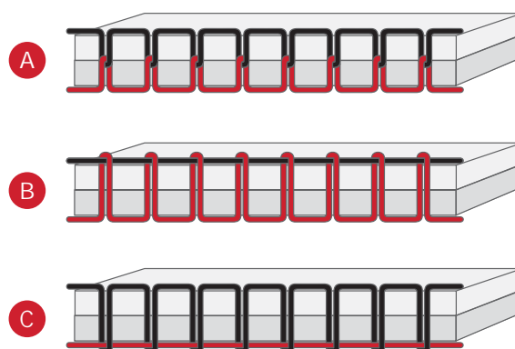
A. Correct tension B. Tension too tight C. Tension too loose
