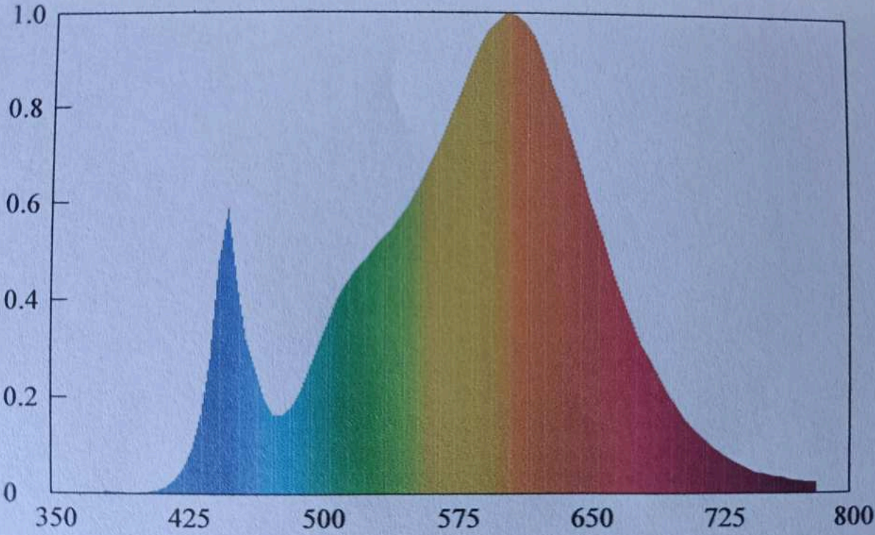
Spectral Distribution
